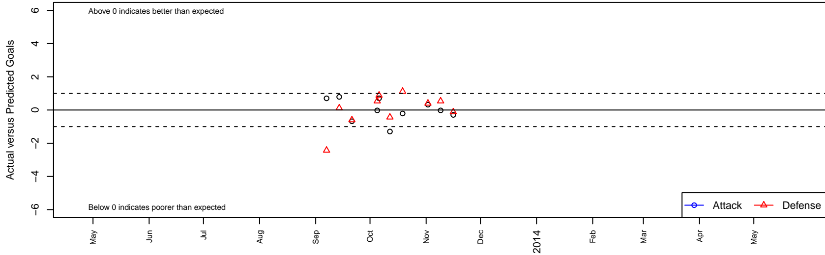
ACC Mavericks Dynamite G01 Dots are actual minus expected GF (blue circles) and GA (red triangles). Blue line is smoothed change in attack strength. Red is smoothed change in defense strength.
